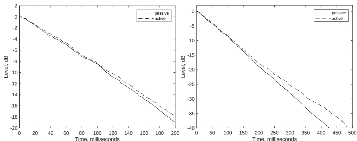
Figure 3: Sound level decays measured at receiver 6.3m from the source with the active acoustics system off (passive, solid line) and on (active, dashed line). Left: Measurement to 200ms, Right: to 500ms.
